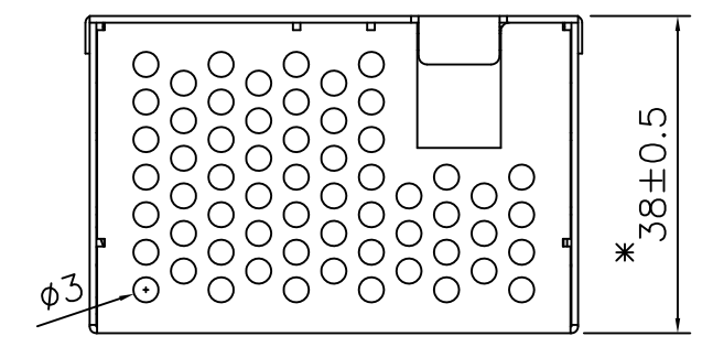
RIGHT-SIDE VIEW
