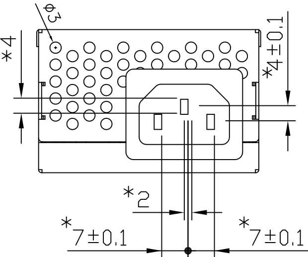
LEFT-SIDE VIEW
